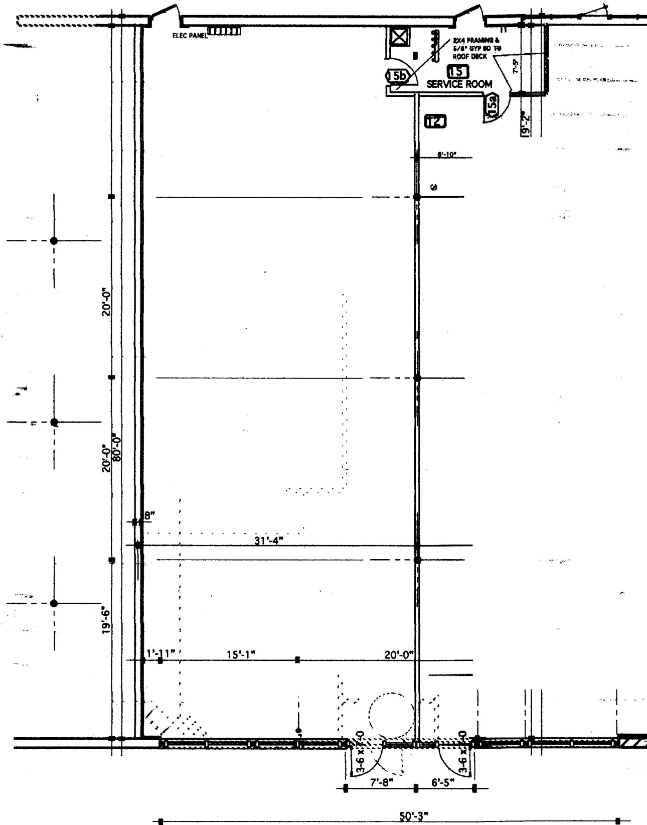
EXISTING PLAN 3/32" = 1'-0"
