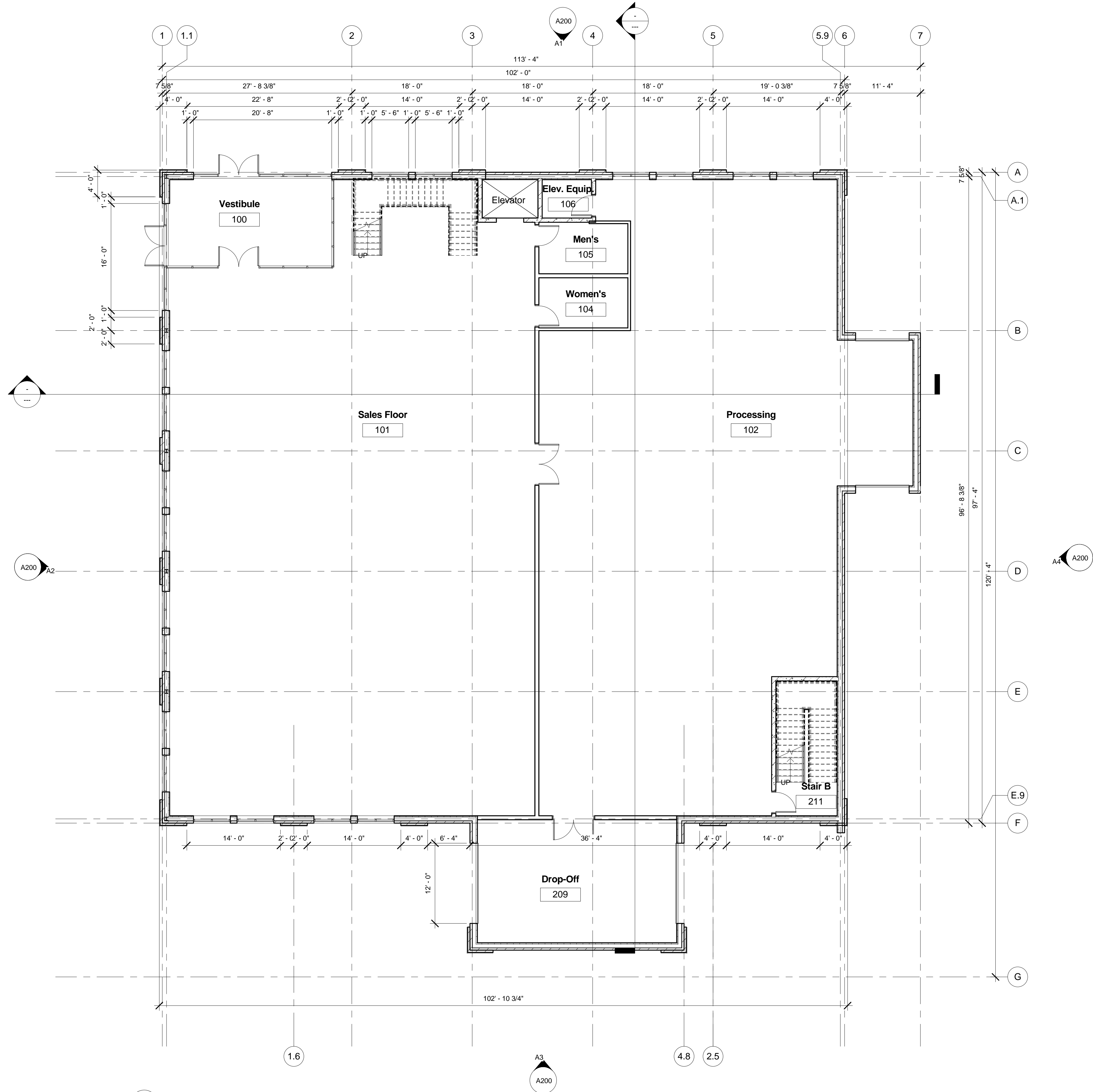
1 FLOOR PLAN - LEVEL 1 1/8" = 1'-0"
