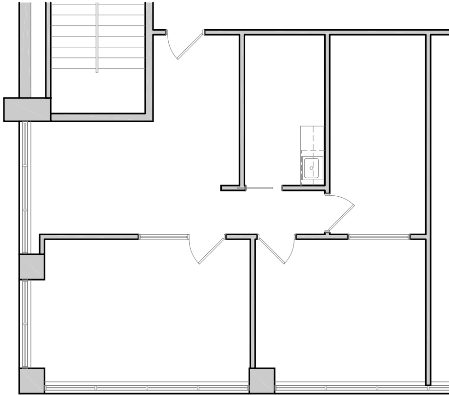
Floor Plan - 1,124 RSF Scale: 1/8" = 1'-0"
