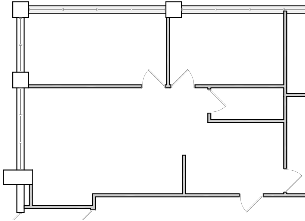
Floor Plan - 1,100 RSF Scale: 1/8" = 1'-0"
